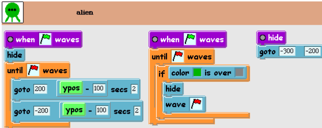
The Alien's Scripts
