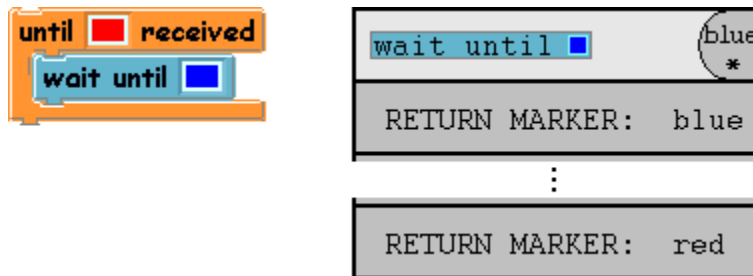
Nested Blocks Waiting for Different Events
