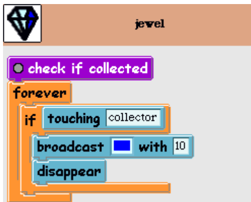
Broadcasting an Event with an Argument Value
