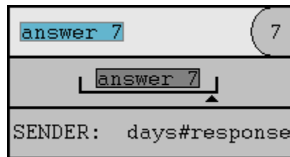
Stack When Evaluating Answer Block
