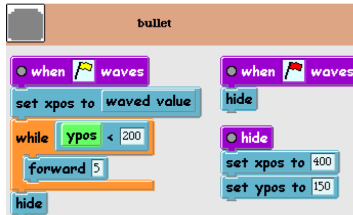
The Bullet's Scripts
